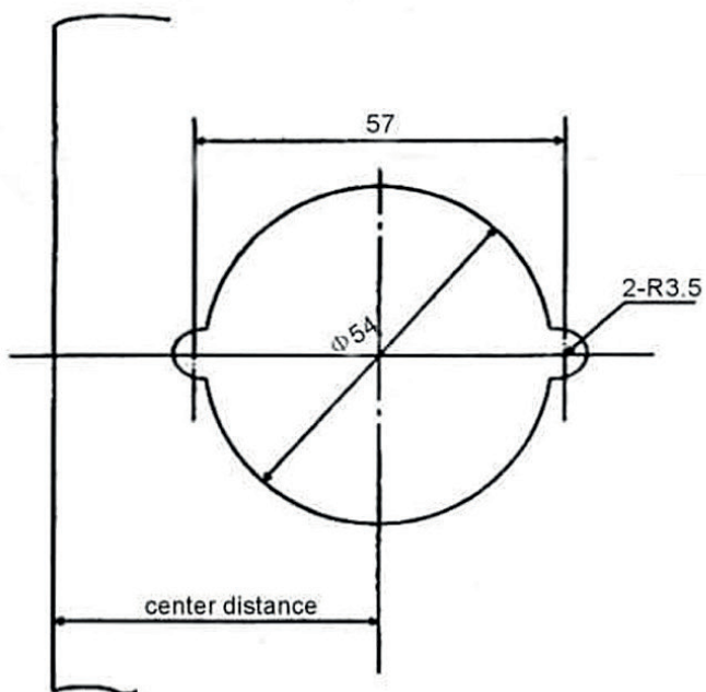
A、 Position of hole for with mounting plate
