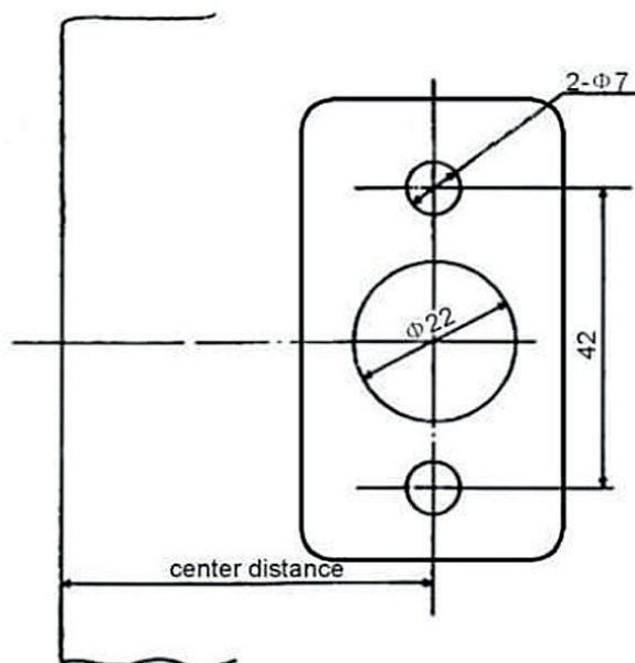
B、 Position of hole for with mounting plate
