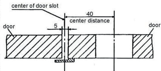
B、 center dimension of dual door
