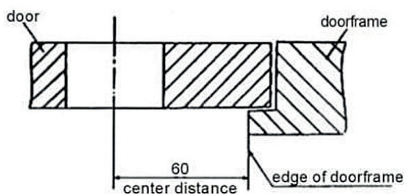
A、 center dimension of single door
