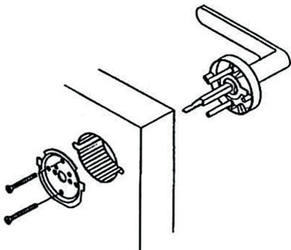
A、 Installation diagram for with mounting plate A
